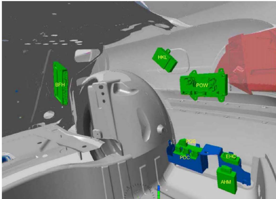
Fig. 61: Overview of control units on right inside luggage compartment
