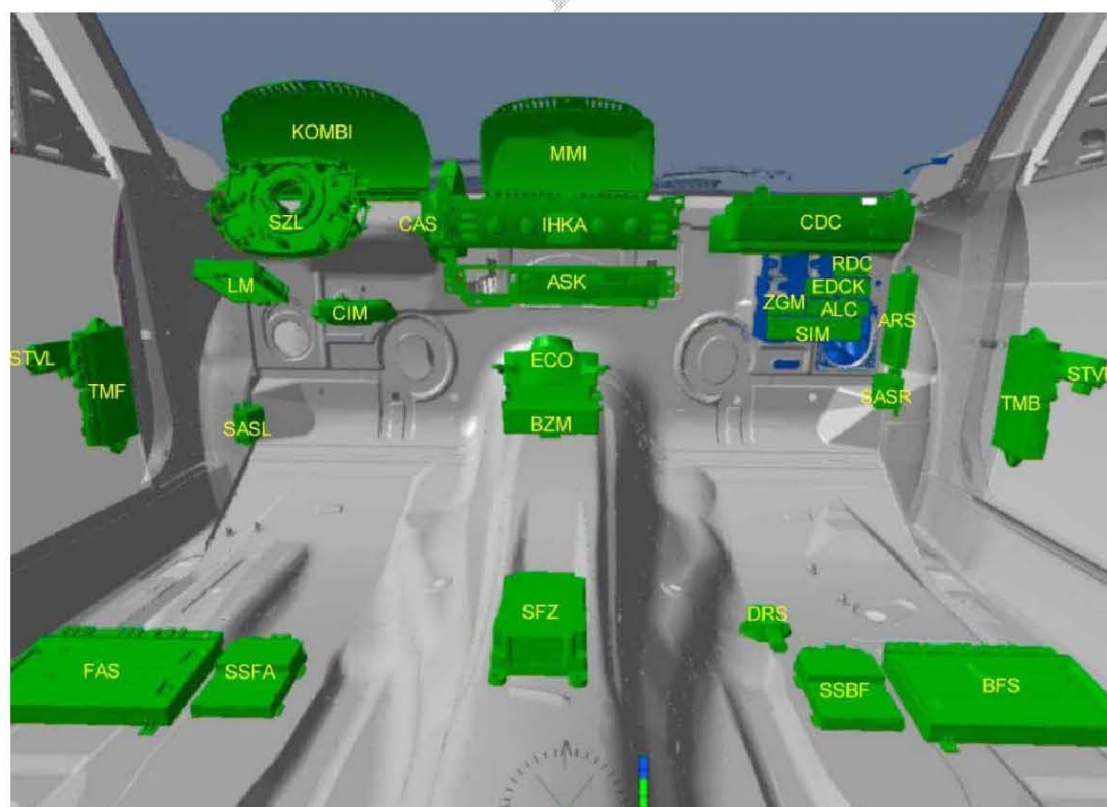
Fig. 59: Overview of control units at front, inside passenger compartment
