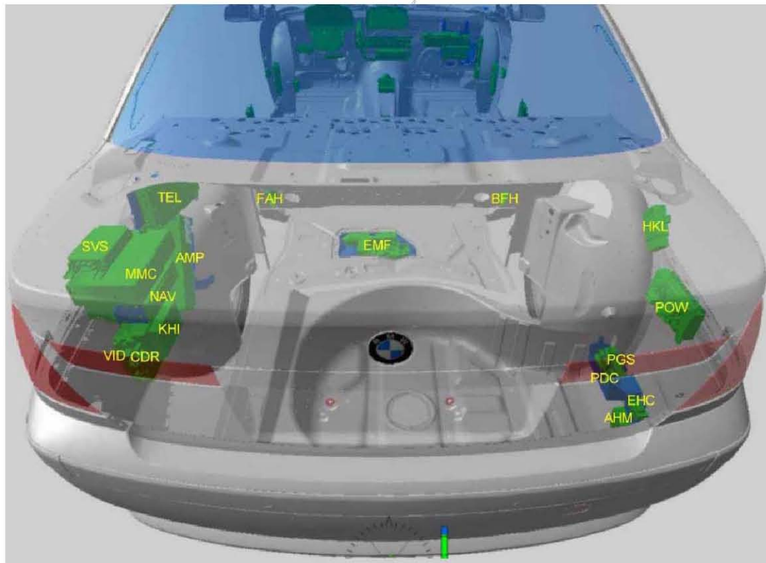
Fig. 60: Overview of control units inside luggage compartment
