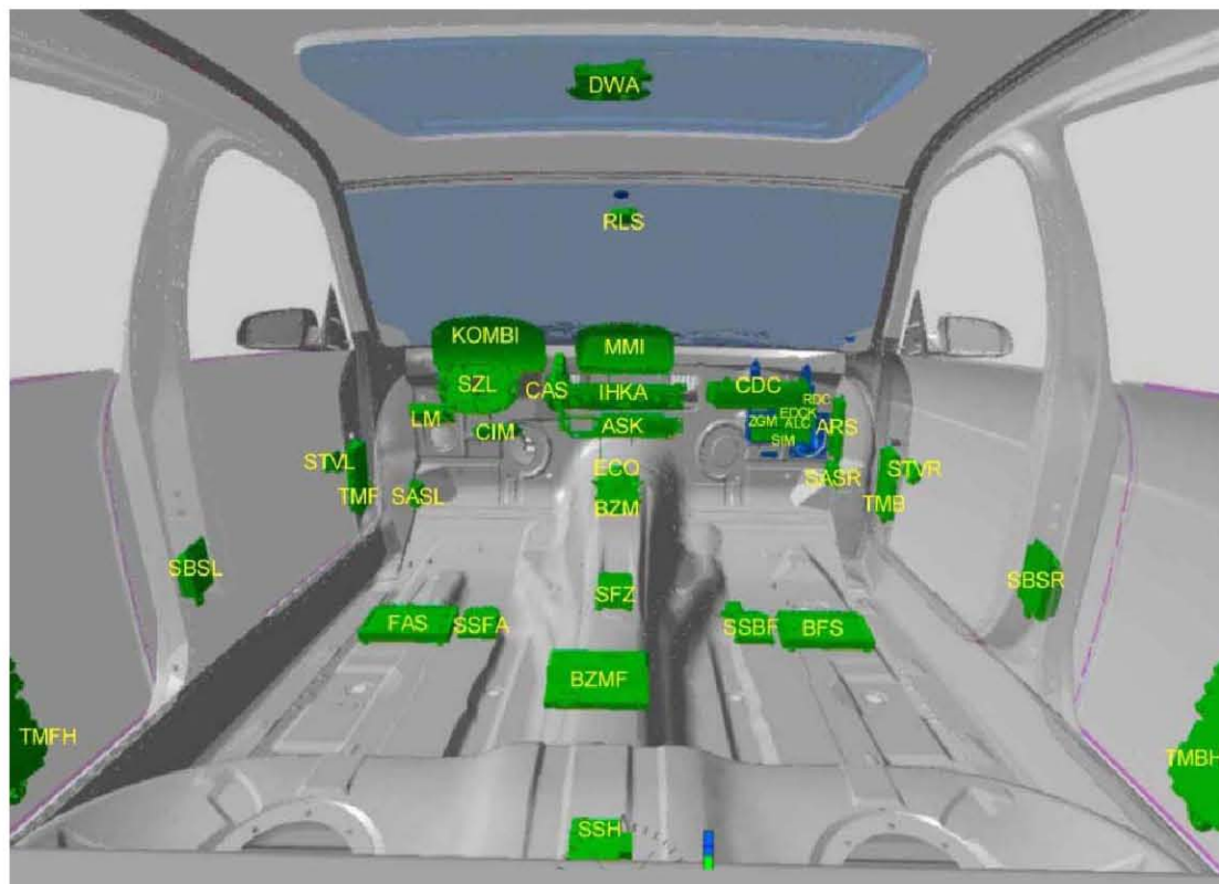
Fig. 58: Overview of control units inside passenger compartment
