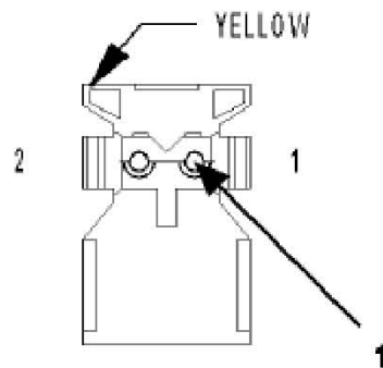
AIRBAG- SIDE CURTAIN- RIGHT
